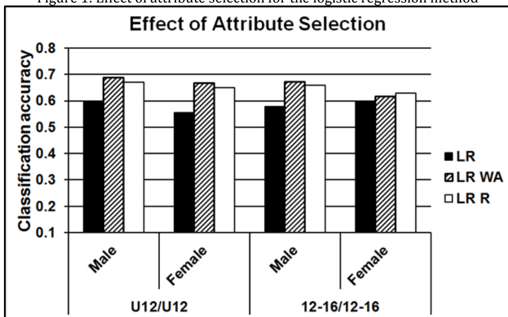
Figure 1: Effect of attribute selection for the logistic regression method
